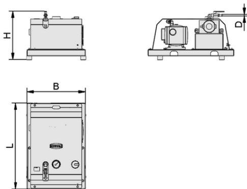
Design data VH-OG Start 10 10
