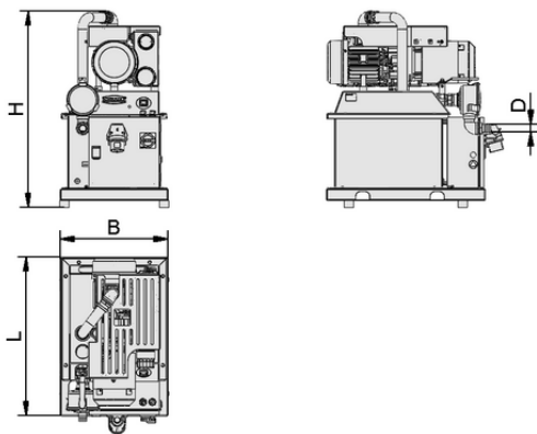
Design data VH-OG Plus 21 30
