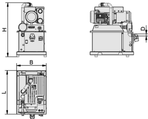
Design data VH-OG Plus 100 100
