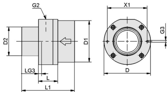
Design data SEC-100 A2
