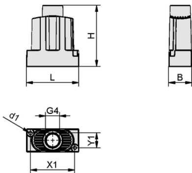
Design data ABL-SET SBPL/SCPL M
