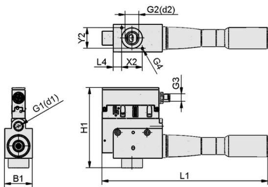
Design data SCPS-L HV 3-20 NC M12-5 PNP
