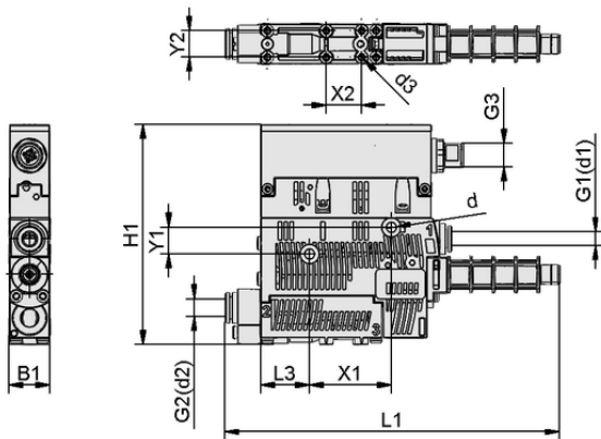
Design data SCPS-UHV-HD 11 G02 NC NPN
