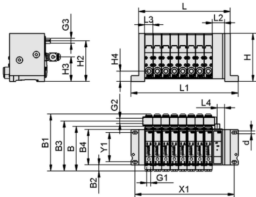
Design data SCTSi EIP E4
