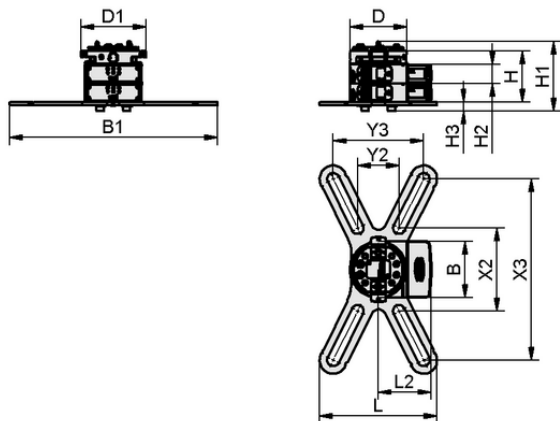
Design data RECBi 24V-DC NC PXR-X 1C MATCH
