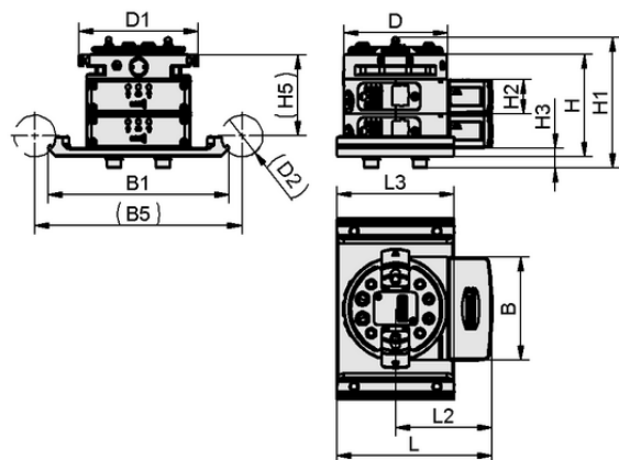
Design data RECBi 24V-DC NC PXT-2 2C MATCH
