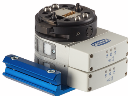
RECBi 24V-DC NC PXT-2 2C MATCH
