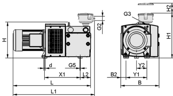
Design data EVE-TR 80 AC3 IE3-TYP2
