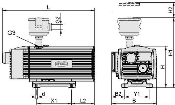
Design data EVE-TR-X 40 AC3 IE3-TYP2 F-VB
