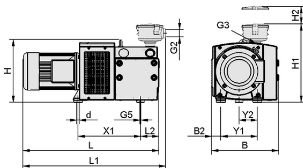
Design data EVE-TR-X 100 AC3 IE3-TYP3 VBV
