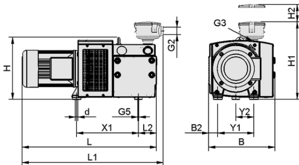
Design data EVE-TR 80 AC3 IE3-TYP4 F
