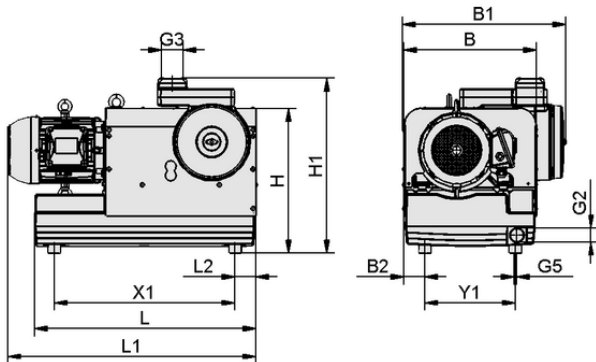
Design data EVE-KL 300 AC3 IE3-TYP4 F
