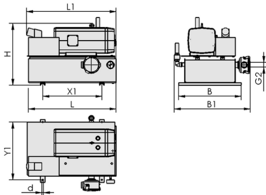
Design data VZ-OG 63 AC3 100 GMS
