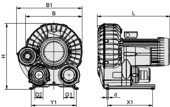
Design data SB 160 115 0.9 IE3-TYP2
