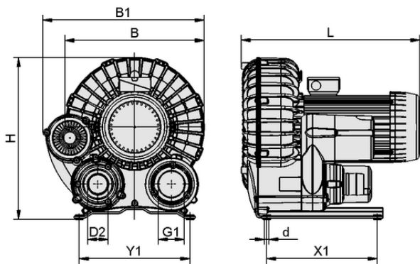
Design data SB 390 245 3.6 IE3-TYP2
