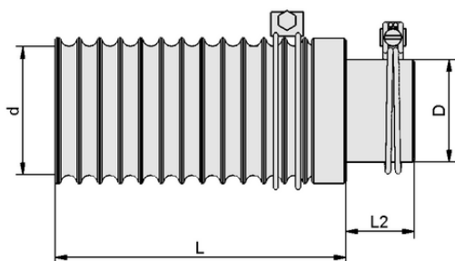
Design data UMR-SET SB Ø76/60
