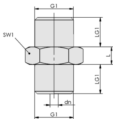
Design data SW 25 G1/8-AG
