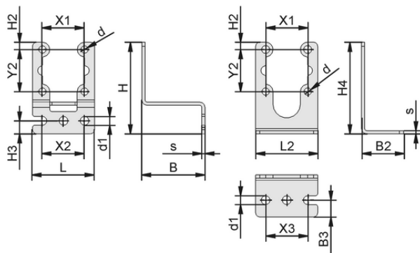
Design data BEF-WIN 30x43.5x29.5 1.5
