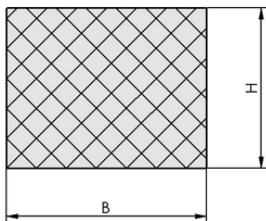
Design data DI-PROF 10x6 MOS EPDM-20
