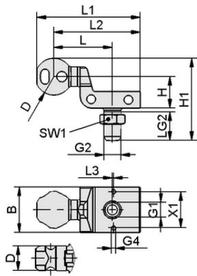
Design data HT-SG A2 E 35 NPT3/8-AG
