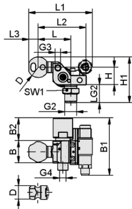
Design data HT-SG A5 I 10 31 NPT3/8-AG AB VS
