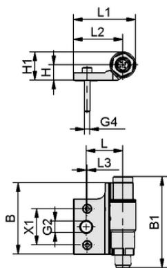
Design data SET HT-SG..E VSi-HD M4x30
