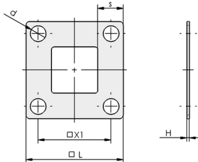
Design data DI-RA 40 PPTA MO-PROF
