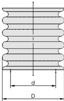
Design data VSL 41-35 PVC-PS GR
