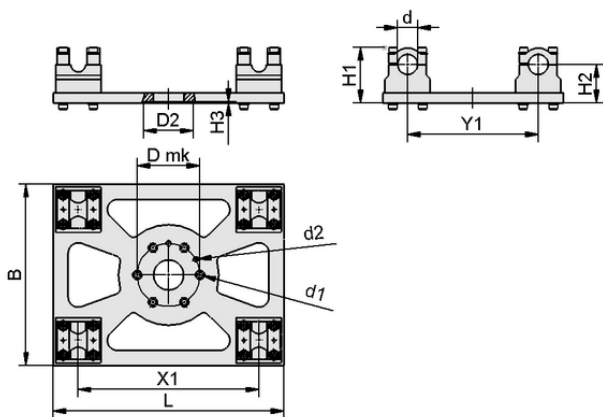
Design data SXT-RF-CL-D-160-60
