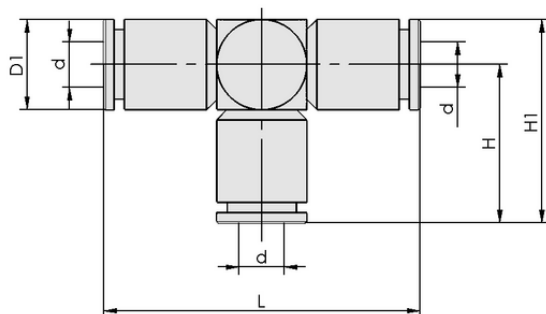
Design data SVB-T 14
