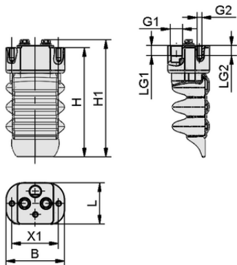
Design data FINGER-MODULE-4C-B-AL-SI-FOOD
