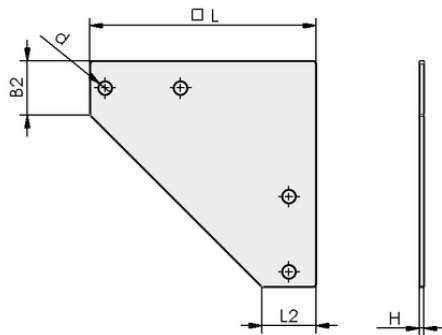
Design data VBR-PR 150x3 E-FL
