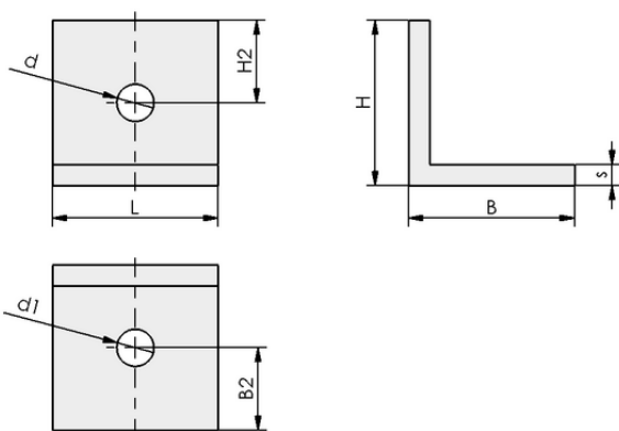
Design data BEF-WIN 40x40x40 5 MO-PROF
