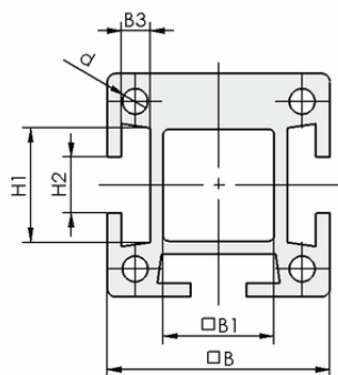
Design data MO-PROF 40 3TN AL-1
