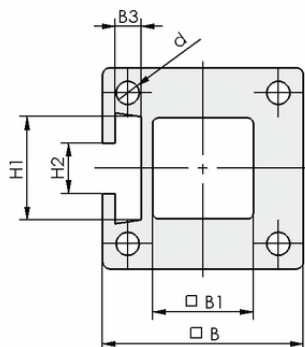
Design data MO-PROF 40 1TN AL-1
